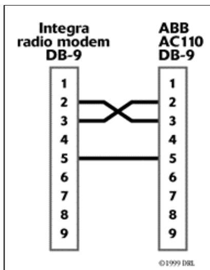
Figure 1: Interface Diagram
